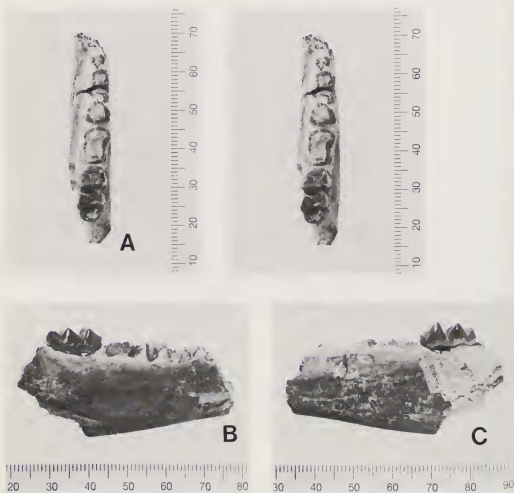
Fig. 1 Isectolophus radinskyi Schoch, new species, YPM 40262 (holotype), right den- tary with M_3 : A, occlusal view, stereo pair; B, labial view; C, lingual view. Scales are in mm.
